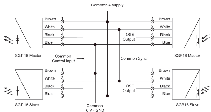
SG 16 OSE Master/Slave wiring
