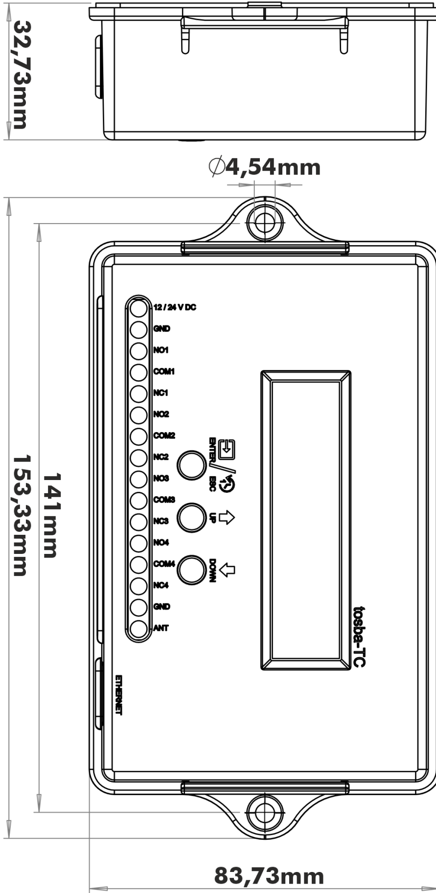
Figure 16 - Dimensions (mm)
